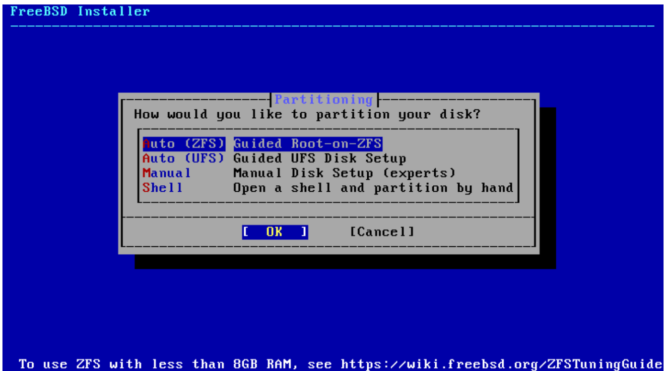
Figure 11. Partitioning Choices
